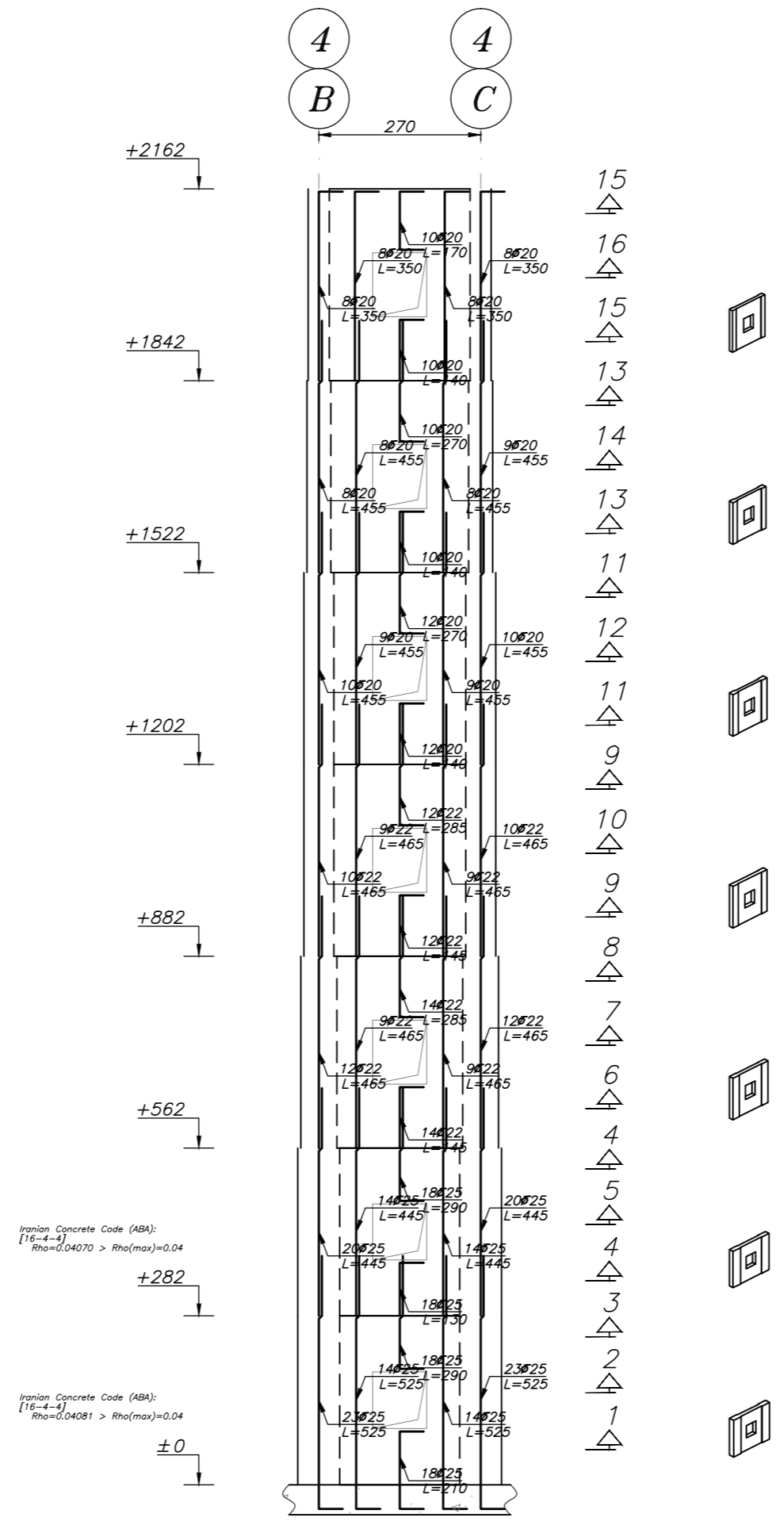
W-1 Scale 1:100
