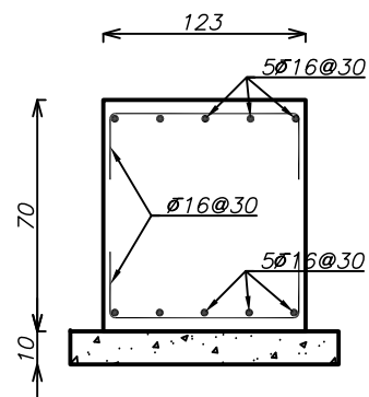
Section F-F
