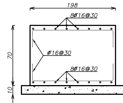
Section E-E
