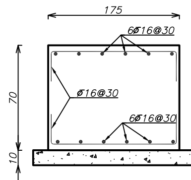
Section G-G
