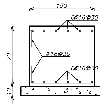
Section H-H
