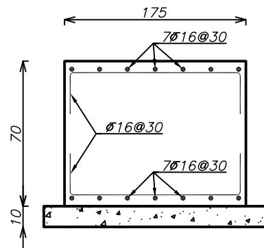
Section C-C
