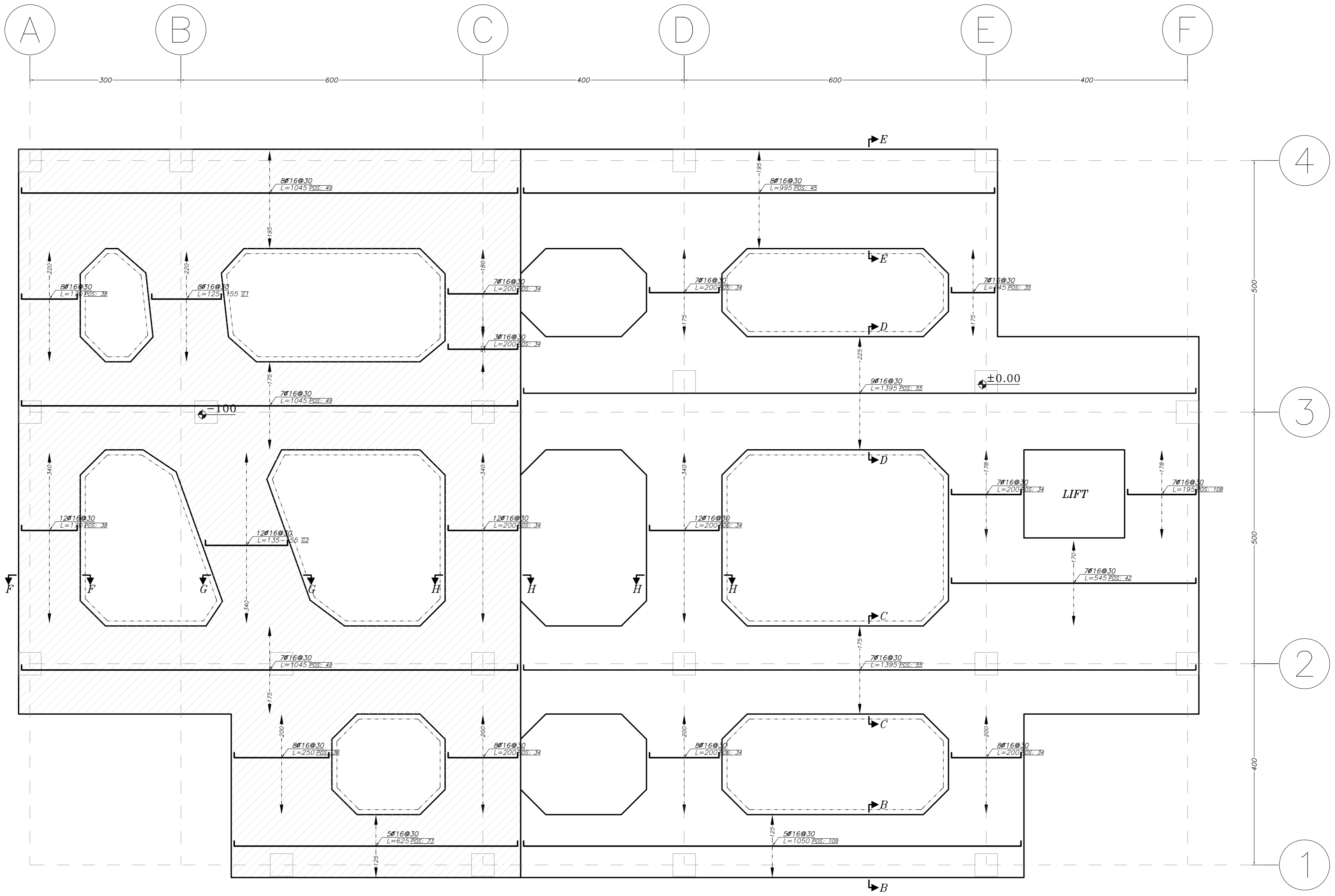
Foundation Main Bars (Top) Scale 1:50 Layer A
