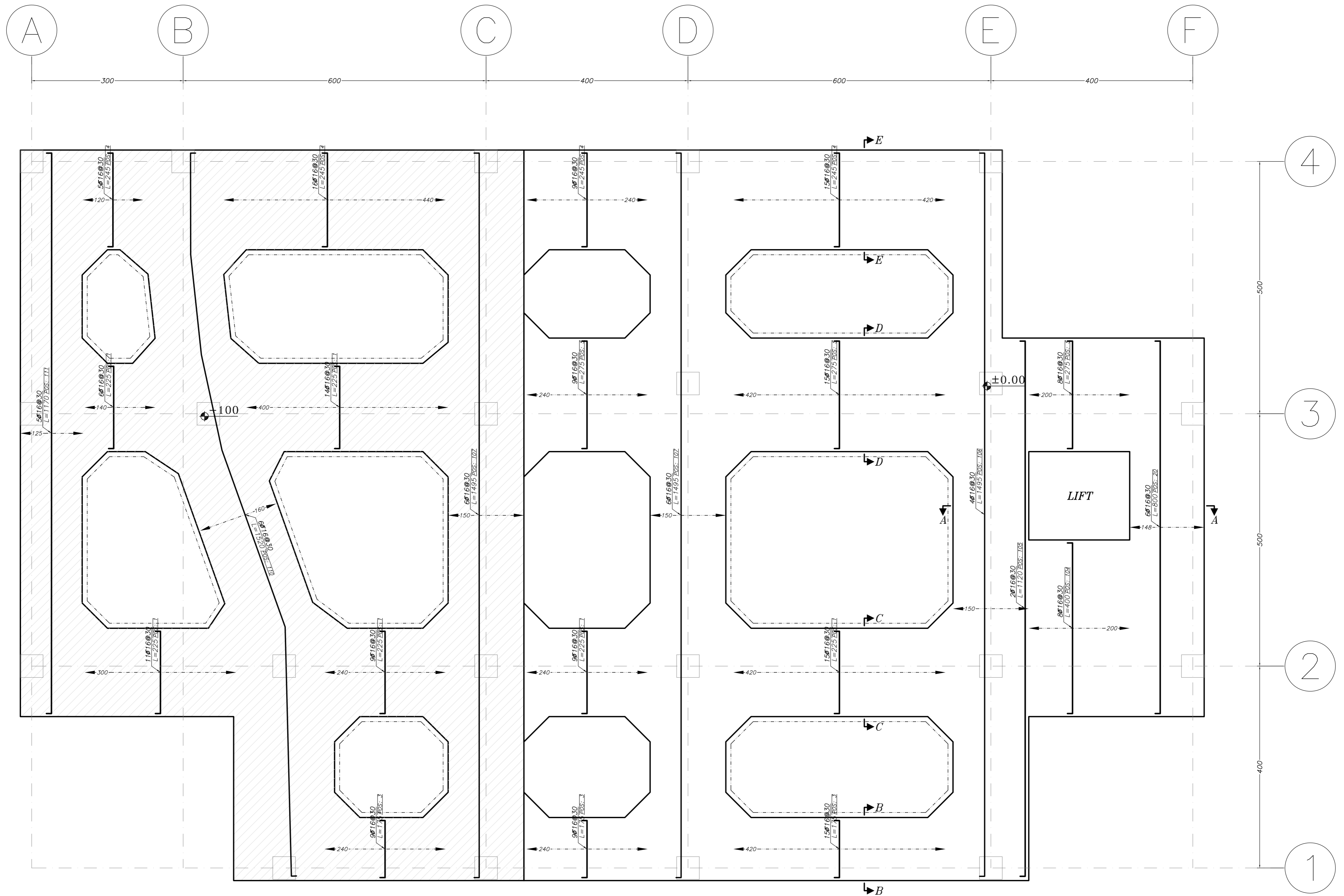
Foundation Main Bars (Top) Scale 1:50 Layer B
