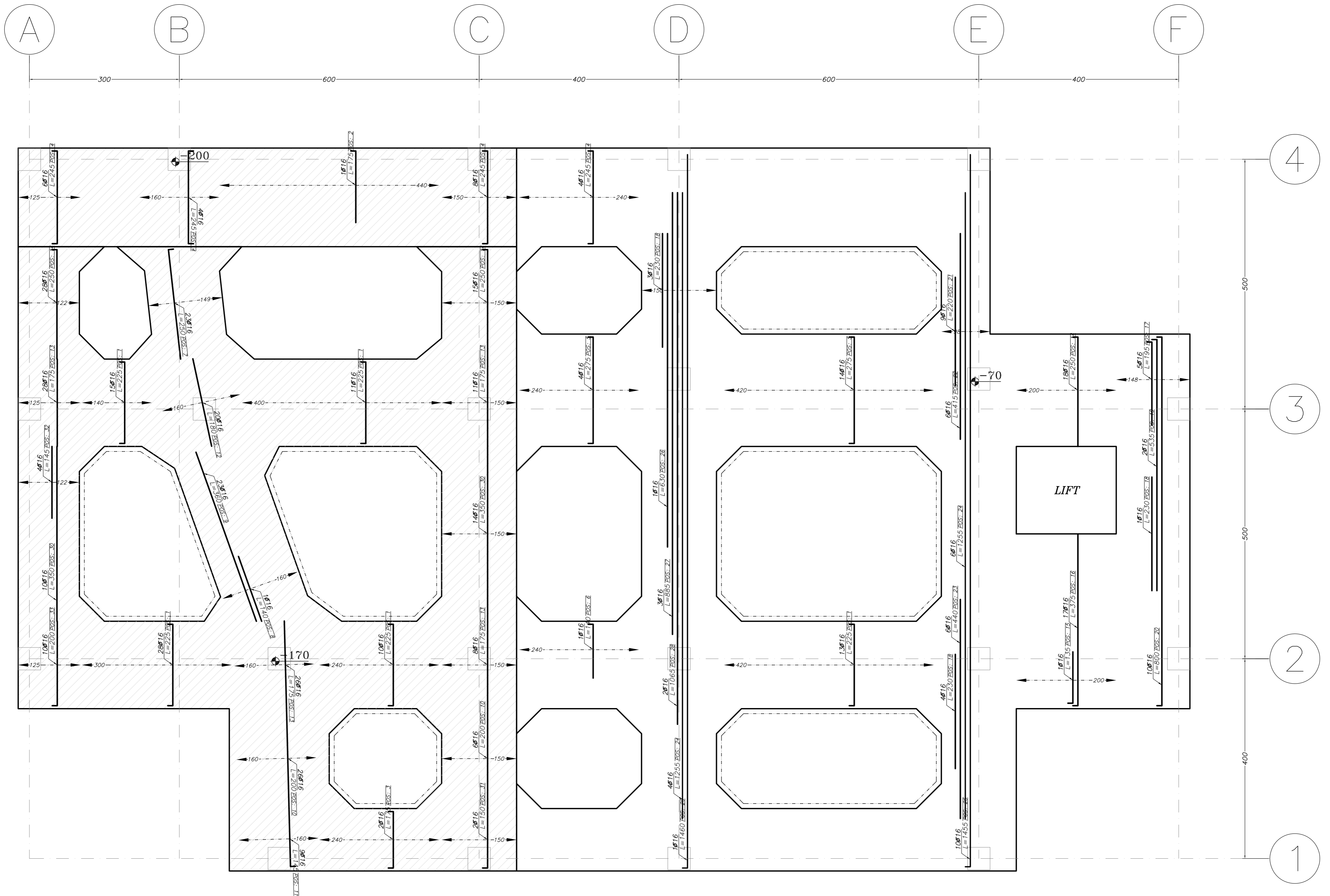
Foundation Added Bars (Bottom) Scale 1:50 Layer B
